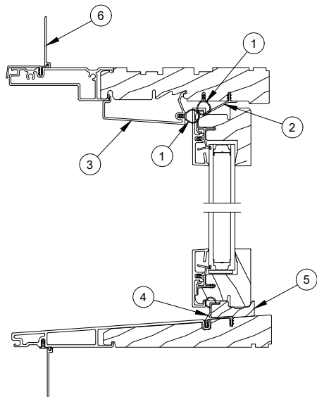
Head Jamb and Sill
