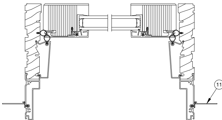
Stationary Jamb Detail
