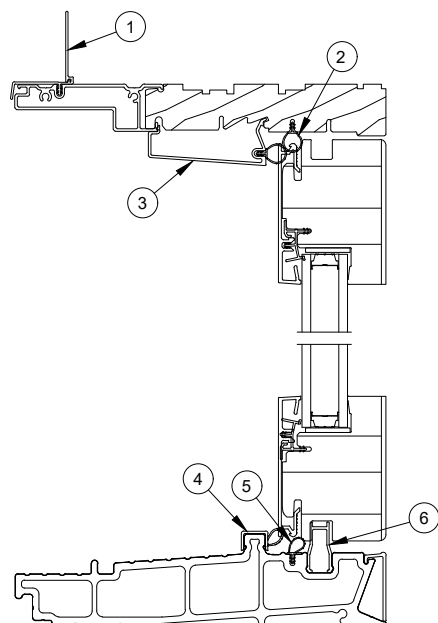
Head Jamb and Performance Sill Detail
