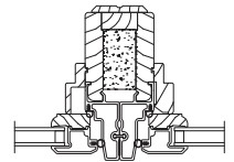
Vertical Mullion
