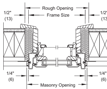
Operator Jamb
