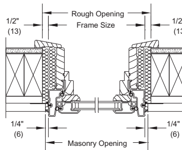
Stationary Jamb
