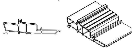
Sill, 6 9/16\", Pre 2014, F2051
