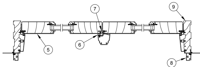
2 Panel Transom
