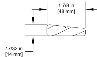
W11177, Spacer Block Clad Part Stop Used between 2011 and 2014
