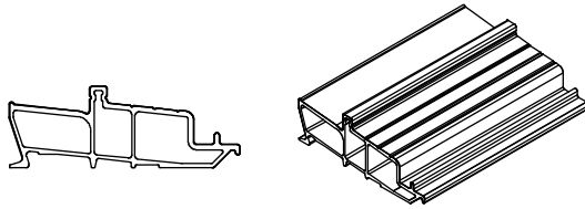
Sill, 4 9/16\", Pre 2014, F2050
