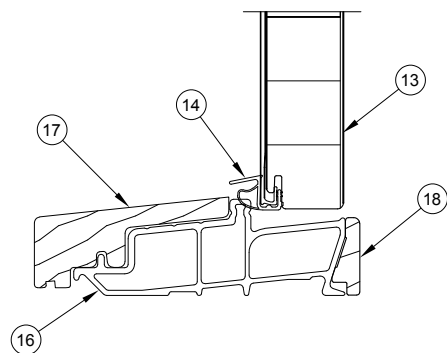
4 9/16" Sill Options
