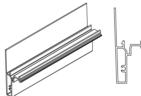
Mull Cap Swinging Screen, A2049
