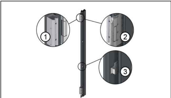
Figure 212 Outswing Hinge Jamb: Mull fillers, hinges, and panel alignment bolts are factory installed. Supports for hardware are fastened through the back of the jamb.
