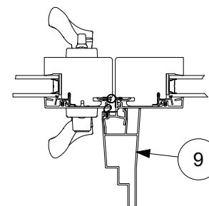
6 9/16" Jamb - 2 1/4" Panel
