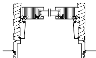
Single Panel Transom Jamb
