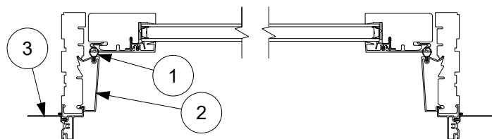
O - 4 9/16" Jambs - 1 3/4" Panel
