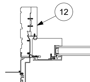
6 9/16" Jambs - 2 1/4" Panel
