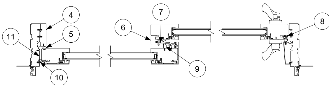
OX - 4 9/16" Jambs - 1 3/4" Panel
