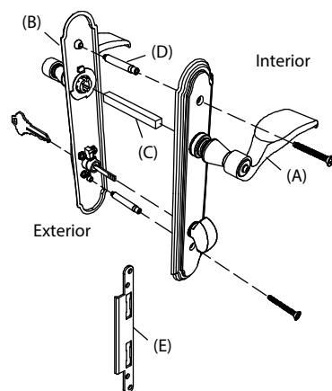
Multi-Point Handle, Active, Solid Brass - Pre 2000 (Essve)
