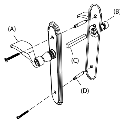
Multi-Point Handle, Inactive, Solid Brass - Pre 2000 (Essve)
