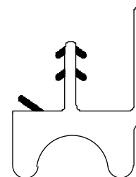
Panel Drip (In-Sash Transom), V800
