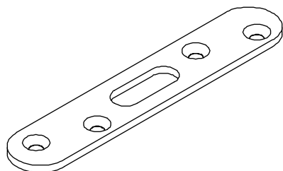
Strike, Inactive Panel, Head Jamb; Multi-Point Lock (Essve) - Pre 2000
