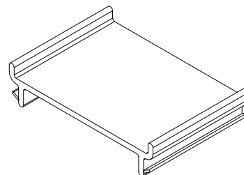
Interior Mull Carrier, MRF, V03544 Casement, Awning, Direct Glaze Rectangle
