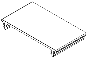
Interior Mull Cover, MRF, V03516 Casement, Awning, Direct Glaze Rectangle
