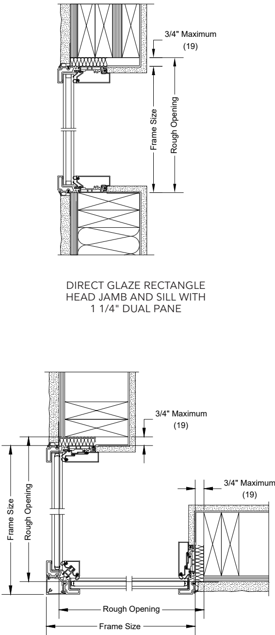
DIRECT GLAZE RECTANGLE CORNER UNITS
