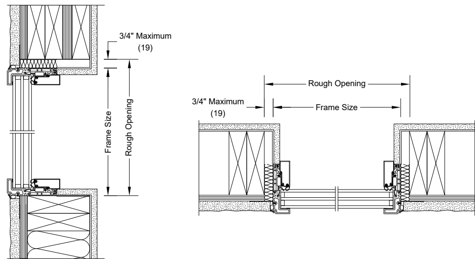
DIRECT GLAZE RECTANGLE HEAD JAMB AND SILL WITH 1 9/16" TRIPLE PANE
