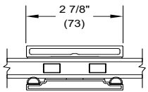
2 7/8" SDL 15/16" Dual Pane
