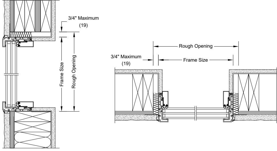
DIRECT GLAZE POLYGON HEAD JAMB AND SILL WITH 1 9/16" TRIPLE PANE
