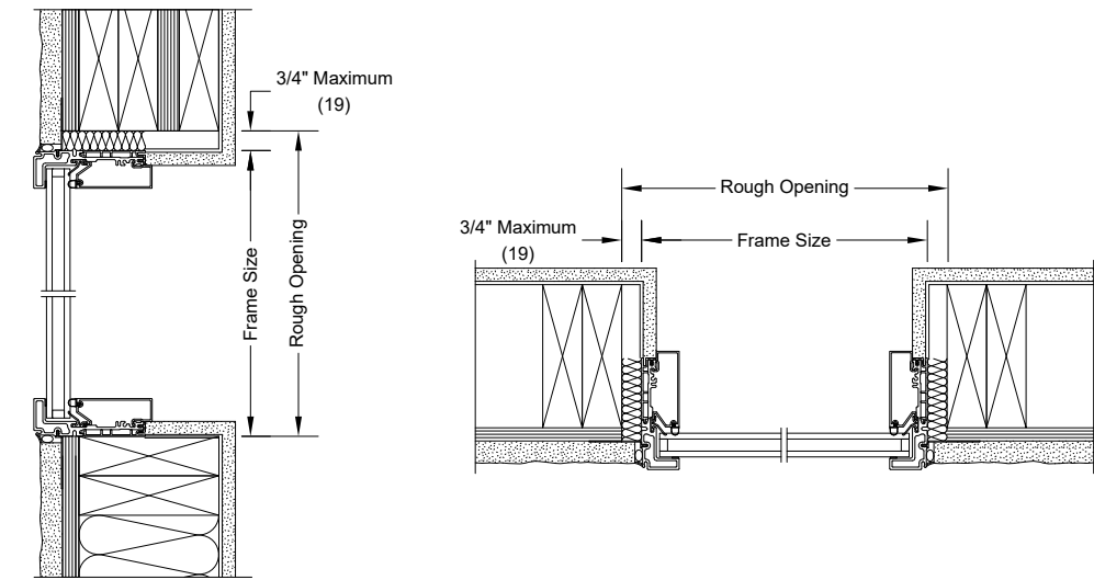
DIRECT GLAZE RECTANGLE HEAD JAMB AND SILL WITH 1 1/4" DUAL PANE
