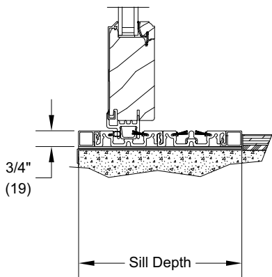
Flush Sill
