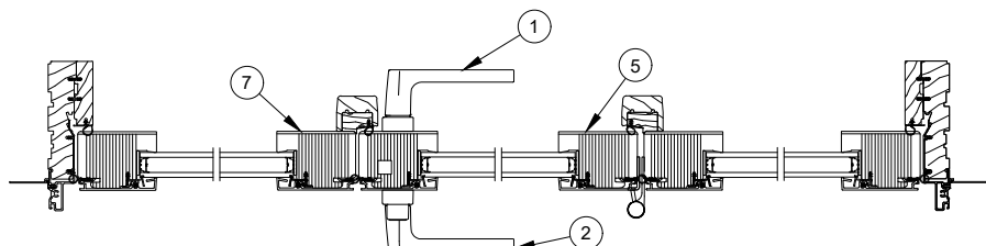
3 Panel Operating Jamb OXO L
