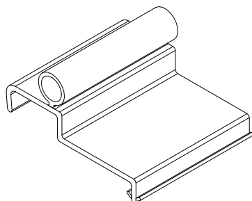
V3133 Top Rail Weather Strip Used on Transom
