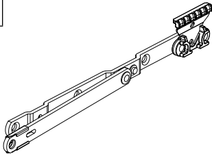
10" Hinge Arm
