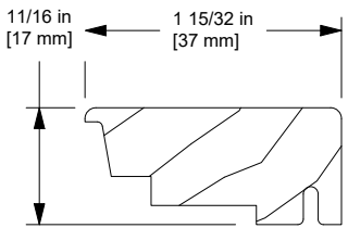
Head Jamb Stop Stationary, W11312
