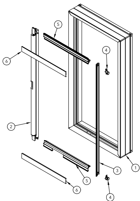
Ultimate Push Out Casement
