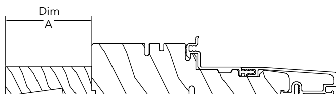
Overall Jamb Width Dimensions
