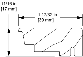
Jamb Stop, Stationary, W11311
