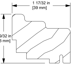
Stationary Solid Wood Jamb Stop, W9790
