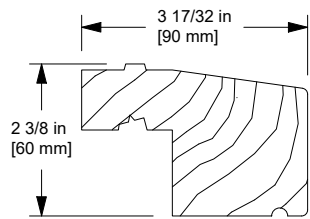
Extended 2” Simulated Thick Sill, W10341
