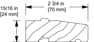
Subsill, W10333
