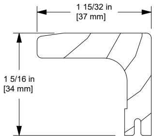
Sill Cover, W10329
