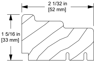
Optional Solid Wood Stop, W10759
