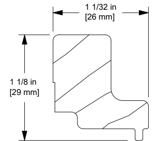
Sill Support Block, W10696
