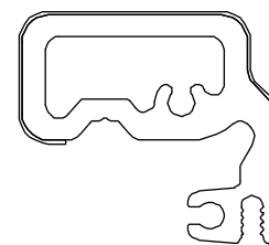
Pull Bar, C0134
