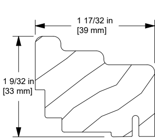
Head Jamb Stop, W9767
