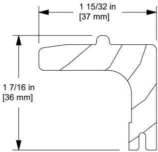
Sill Cover, W9788
