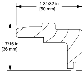
Sill Cover, W10667
