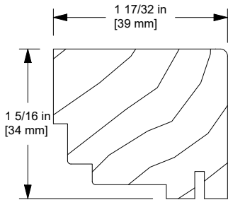
Sill Cover, Stationary, W10454
