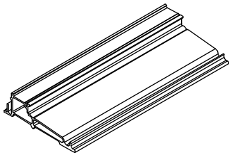
Ultrex Sill, 4 9/16" Jamb, Inswing, F256
