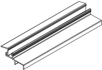
Stationary Panel Drip/Sill Spacer, Inswing, V941
