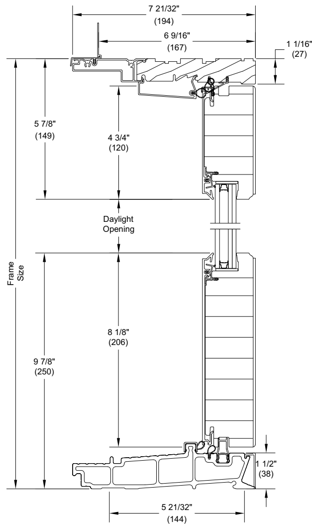
6 9/16" Head Jamb and Sill
