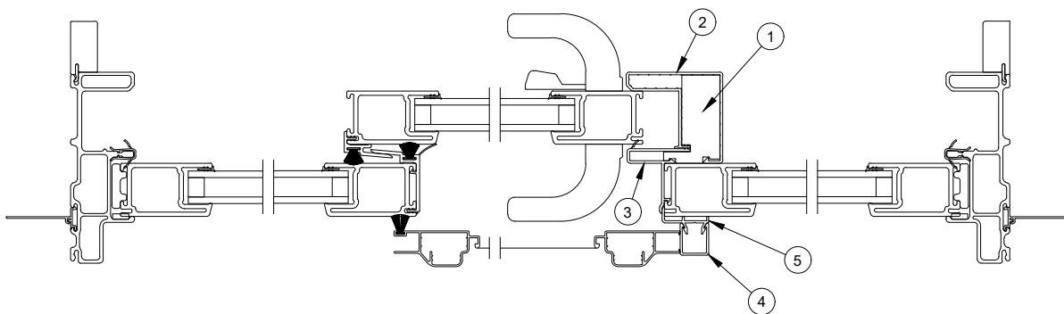
Jamb Detail 3-Panel OXO
