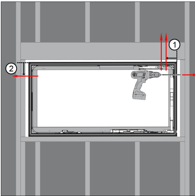
Figure 3 Awning: red arrows denote factory installation holes.
