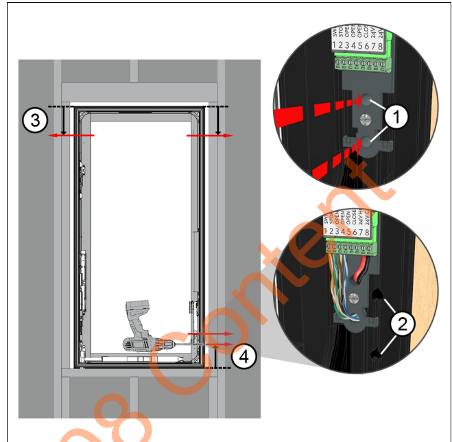
Figure 1 Casement: red arrows denote factory installation holes.
