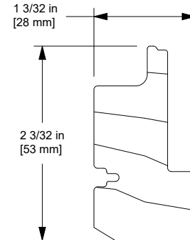
W11906 Transom Cover, Interior
