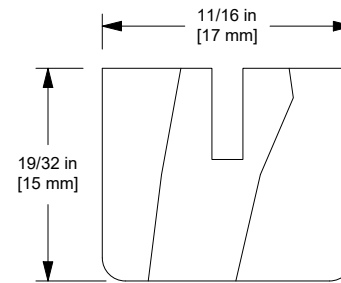
W12224 Parting Stop, Round Top
