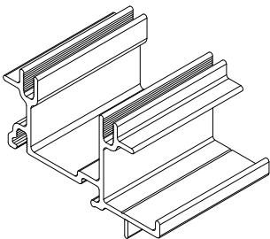
V2432 Mid Exterior Cover Base If the original unit had performance brackets, then a secondary fabrication is needed to accommodate the brackets.
