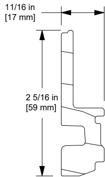
W11581 Interior Jamb Cover
