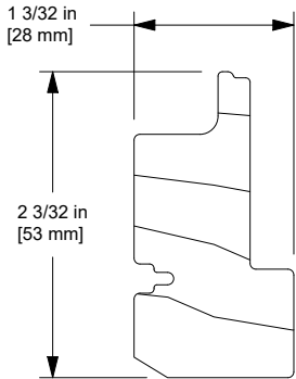
W11906 Transom Interior Cover/ Interior Frame Cover
