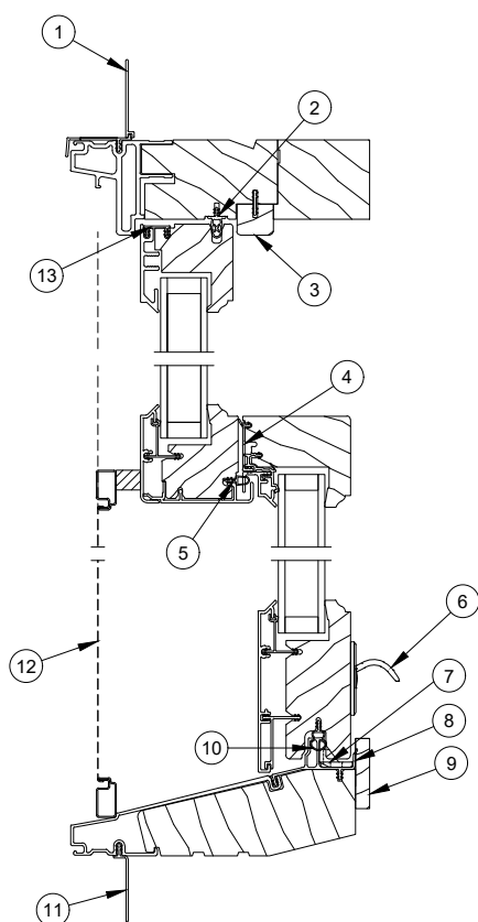
Head Jamb and Sill Details
