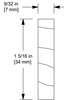
W11576 Sill Liner
