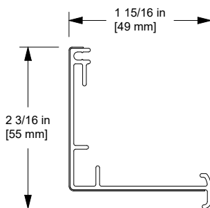
Interior Housing, C0117
