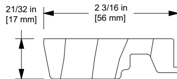
W12061 Transom Sill Filler
