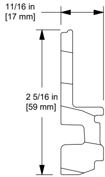
W11581 Interior Jamb Cover/ Interior Frame Cover
