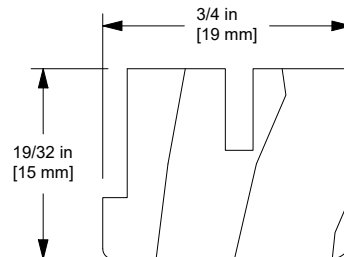
W12851 Head Jamb Stop, Round Top (Picture/Transom)
