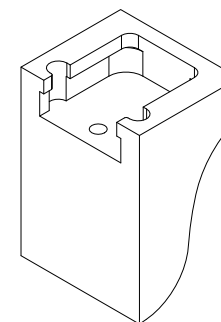
Exterior Sash Lug, Ogee Profile
