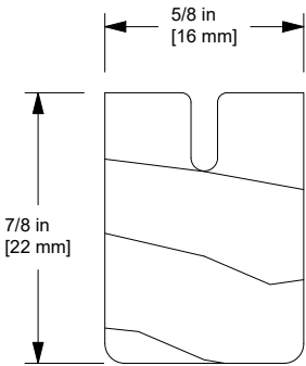
W11578 Parting Stop/ Interior Frame Cover
