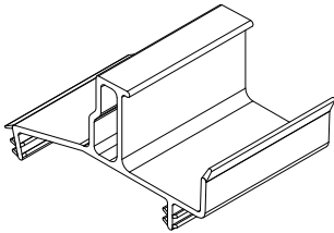
V2191 Sill Thermal Break/Liner NOTE: V2191 for Rectangular products is available in Configured Parts in OMS. For Custom Color Clad, Sill Thermal Break color will match the selected exterior weather strip package color.
