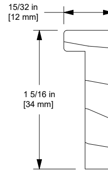
W11825 Sill Liner, Picture/Transom
