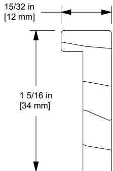
W11825 Sill Liner/ Interior Frame Cover Picture or Transom
