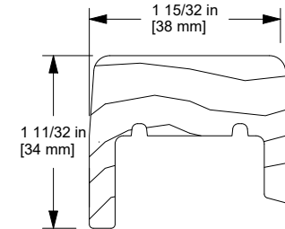
W13631 Astragal Cap, Square
