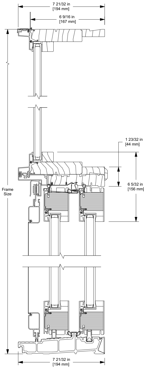
6 9/16 inch Direct Glaze Mull over USD2.25
