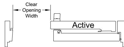
OX - Clear Opening Width Interior Vertical With Exterior Flush Pull Handles
