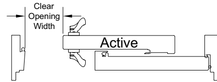
OX - Clear Opening Width Harp Handles
