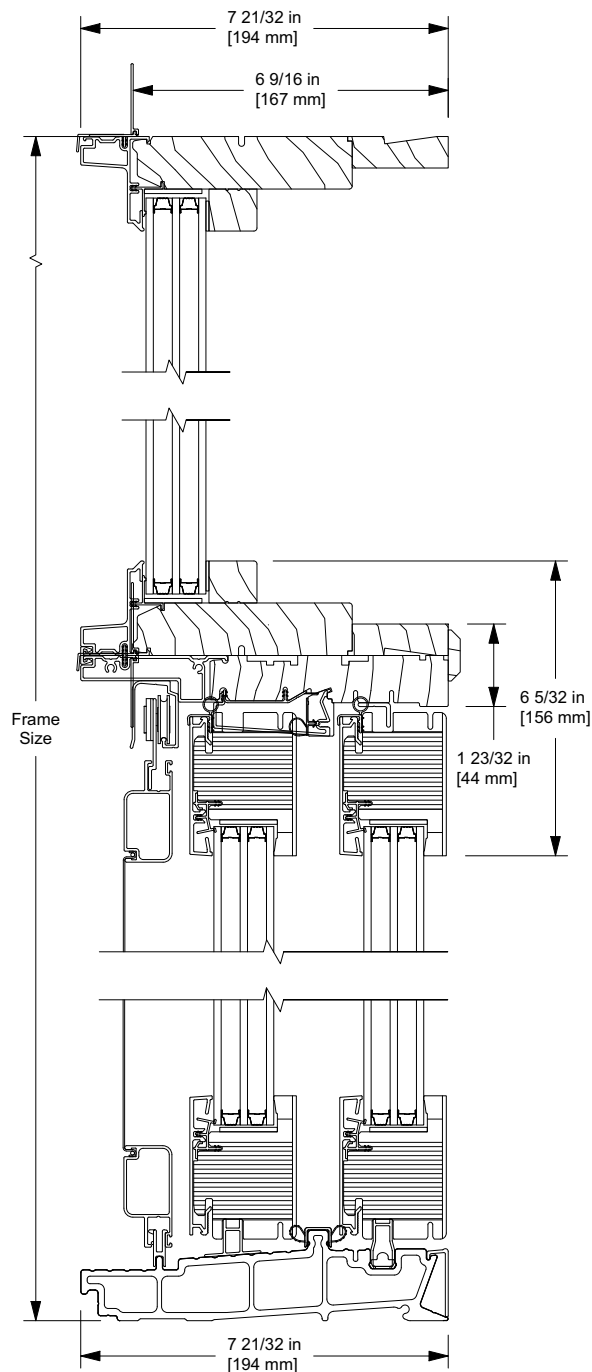
6 9/16 inch Direct Glaze Mull over USD2.25
