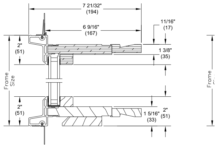
CASEMENT - 6 9/16"
