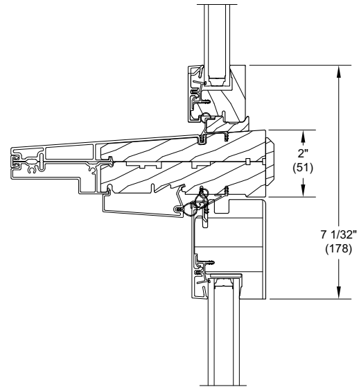
Rectangular Ultimate Transom Over Ultimate In swing Door
